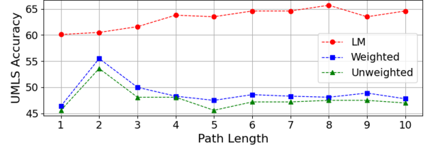
Figure 3. Testing accuracy w.r.t. various maximum pre-training random walk lengths ( 1 \leq L_{max} \leq 10 ) on Countries (left) and UMLS (right) datasets, respectively. For Countries, the LM ( P_{LM} ) performance converges to the weighted aggregation ( P_w ) performance, while for UMLS, LM consistently outperforms both weighted ( P_w ) and unweighted ( P_s ) aggregation performance. This is likely because LM ( P_{LM} ) can learn a better logical rule weighting scheme than weighted aggregation ( P_w ) in more complex KGs.
