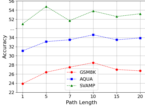
Figure 5. Testing accuracy of continue pre-training with our random walk paths of different length L_{max} . Each line corresponds to a different MWP dataset and thus is not directly comparable. We want to highlight the common trend here that each line would peak at some optimal path length range, which is similar to Figure 4.
