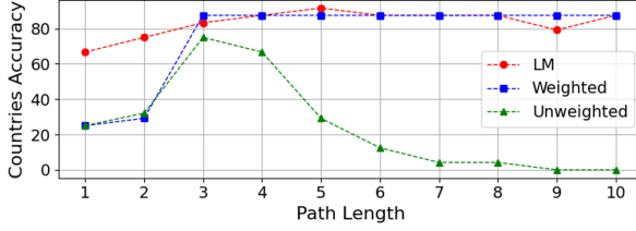
Figure 3. Testing accuracy w.r.t. various maximum pre-training random walk lengths ( 1 \leq L_{max} \leq 10 ) on Countries (left) and UMLS (right) datasets, respectively. For Countries, the LM ( P_{LM} ) performance converges to the weighted aggregation ( P_w ) performance, while for UMLS, LM consistently outperforms both weighted ( P_w ) and unweighted ( P_s ) aggregation performance. This is likely because LM ( P_{LM} ) can learn a better logical rule weighting scheme than weighted aggregation ( P_w ) in more complex KGs.
